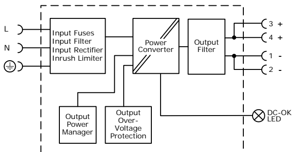
Functional diagram DTM70
