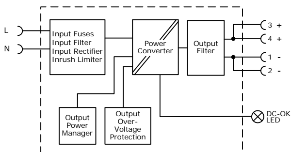
Functional diagram DTM70-C8
