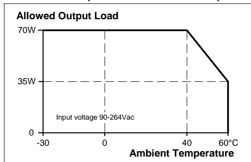
Allowed output load vs. ambient temp.
