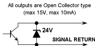
Figure 3–10: Open collector signals are shunted by internal 24V Zener
