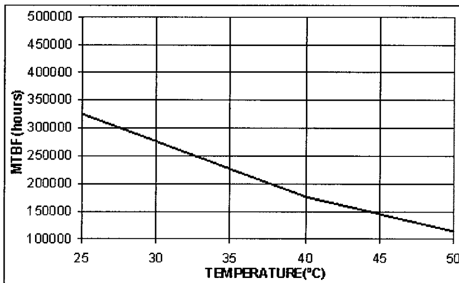
TEMPERATURE CURVE
