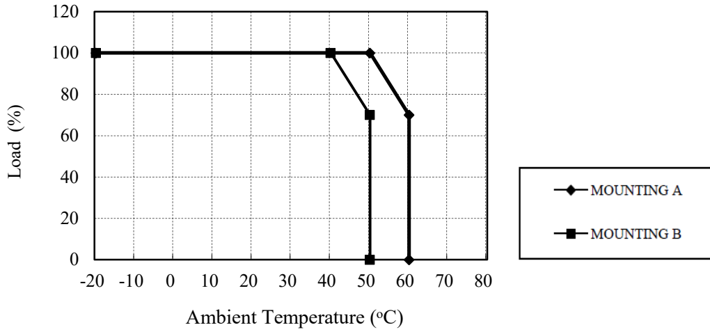
Derating Curve
