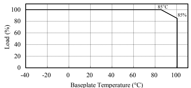
Derating Curve
