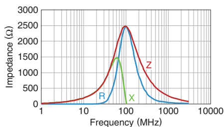
KMZ1608AHR252BTD25
