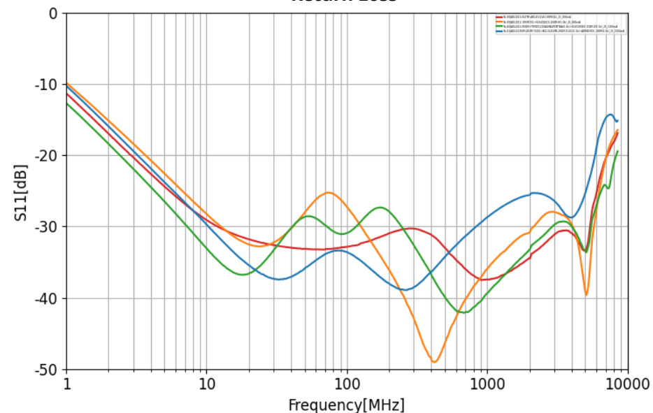
Return Loss
