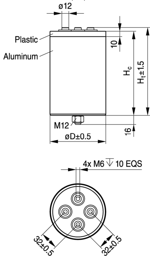
Figure 3: - B25697H – ØD = 100 mm
