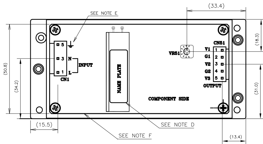
CUSTOMER MOUNTING HOLE INDICATION(TOP SIDE VIEW)
