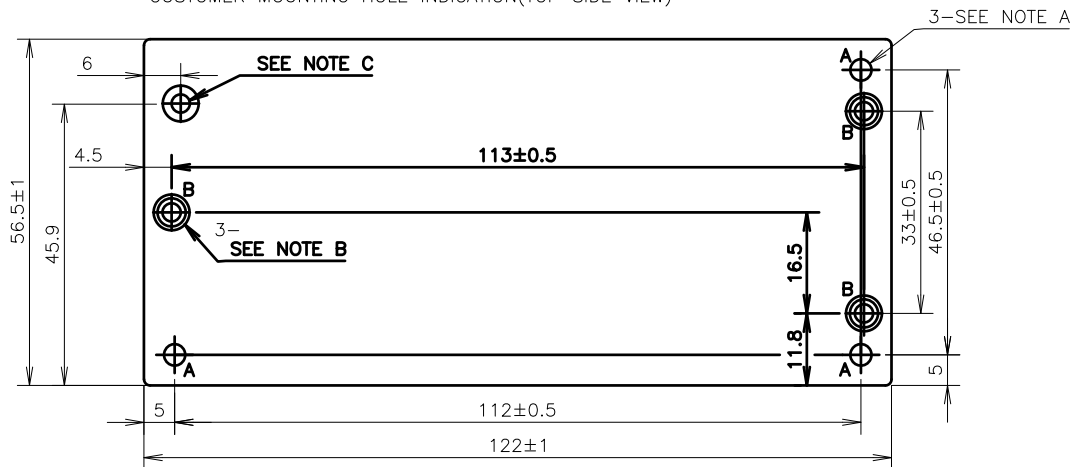
CUSTOMER MOUNTING HOLE INDICATION(TOP SIDE VIEW)
