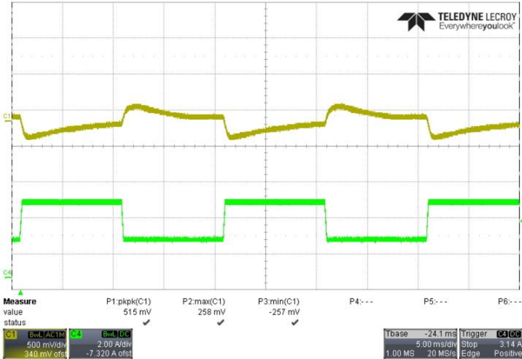
25% to 50% load; 230Vac input
