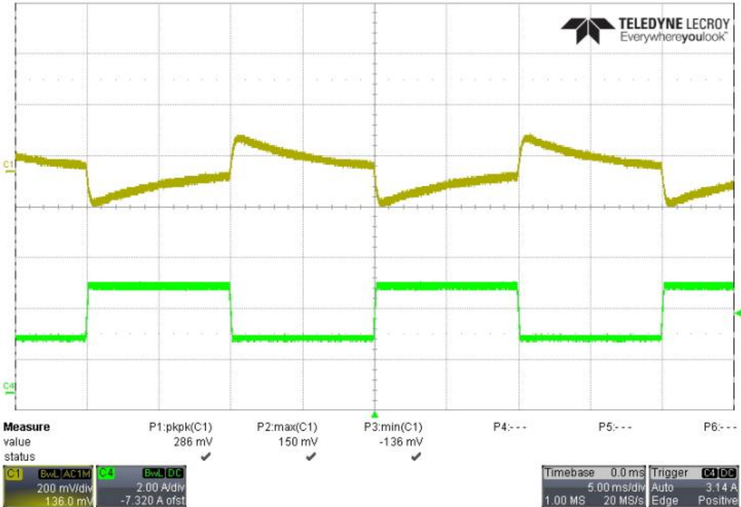
25% to 50% load; 115Vac input
