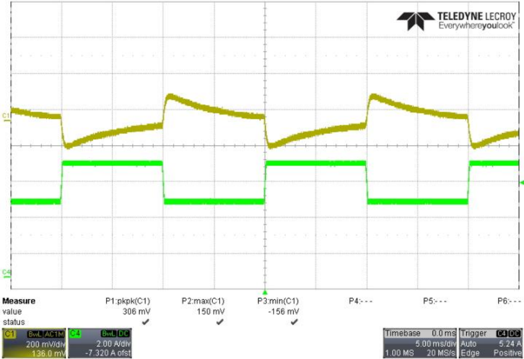
50% to 75% load; 230Vac input
