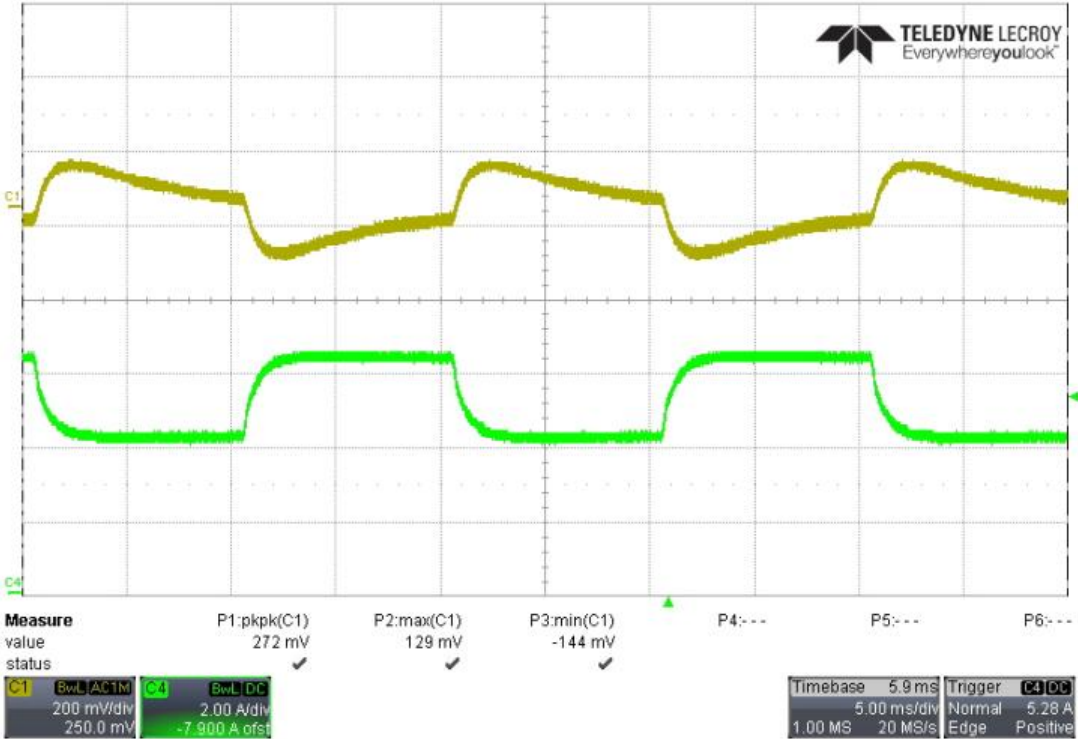
50% to 75% load; with 3950uF capacitance; 230Vac input
