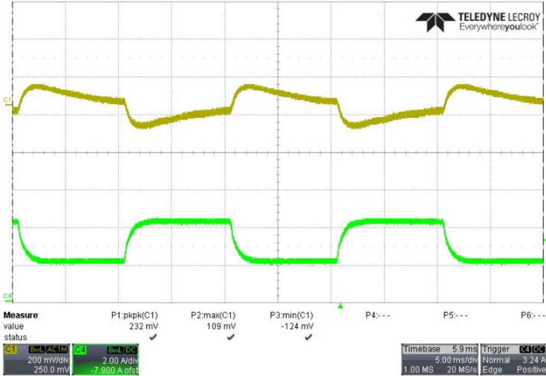
25% to 50% load; with 3950uF capacitance; 115Vac input
