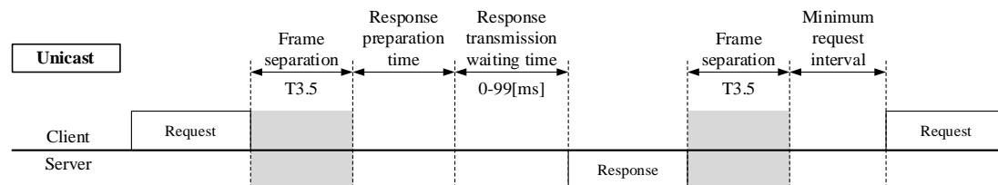
Figure 5-1 Unicast
