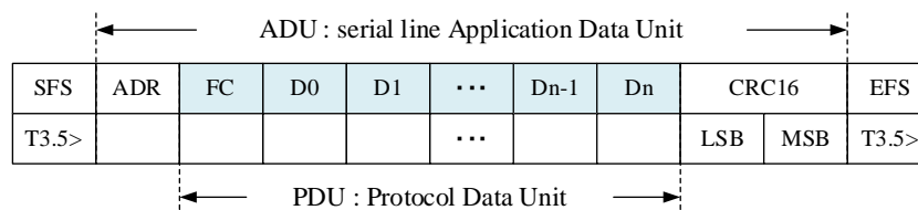
Figure 5-3 Request frame
