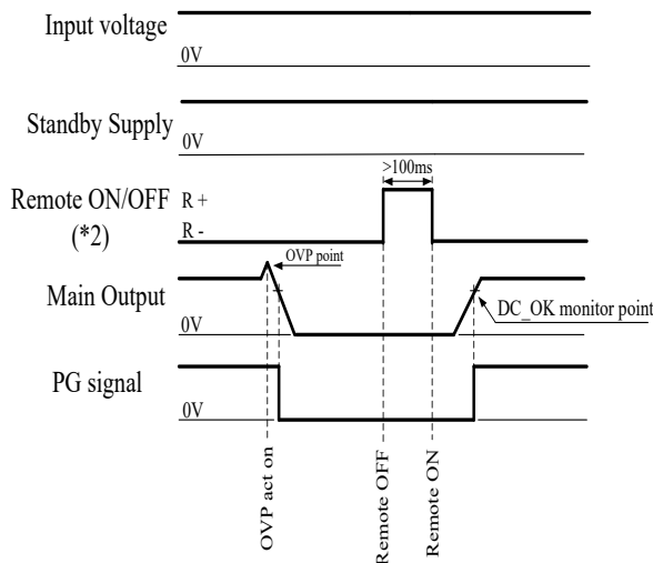
OVP recovery sequence time chart (2)
