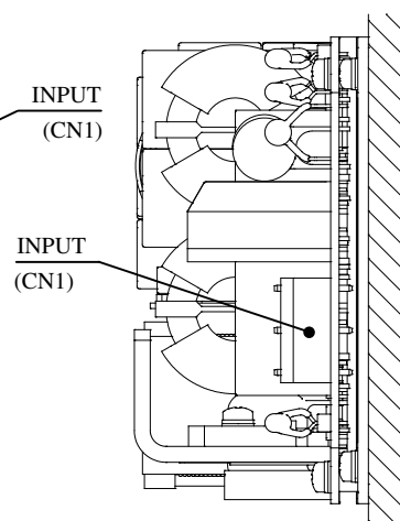
Mounting C
