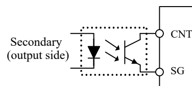
Fig.6-2 CNT Connection (2)
