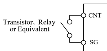
Fig.6-1 CNT Connection (1)
