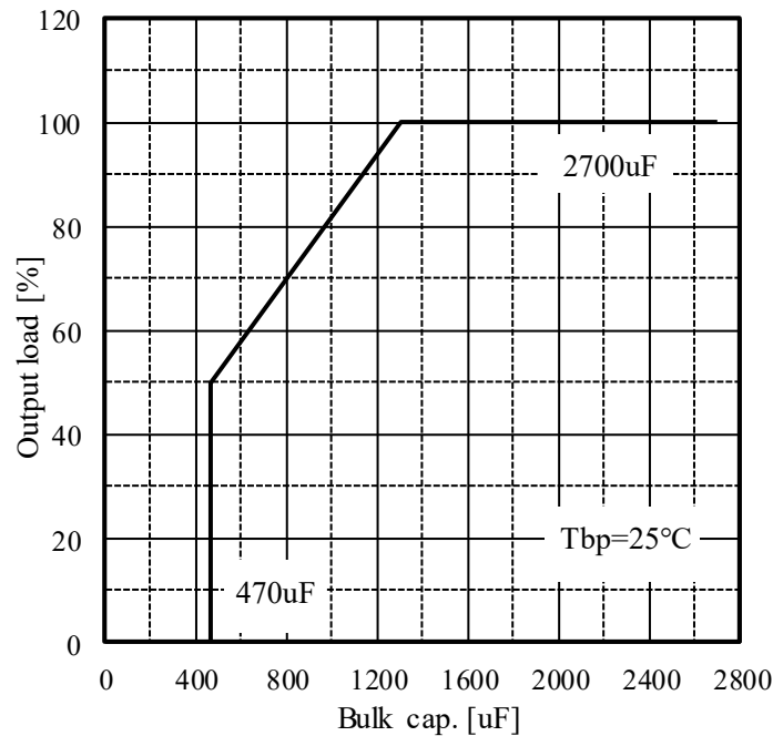
Fig.5-3 Output Load v.s. Boost Bulk Capacitance
