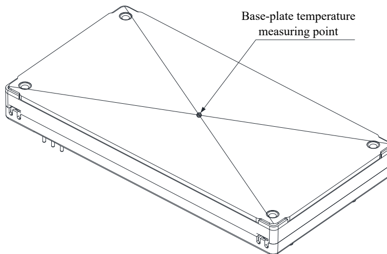
Fig.6-7 Base-plate measuring point
