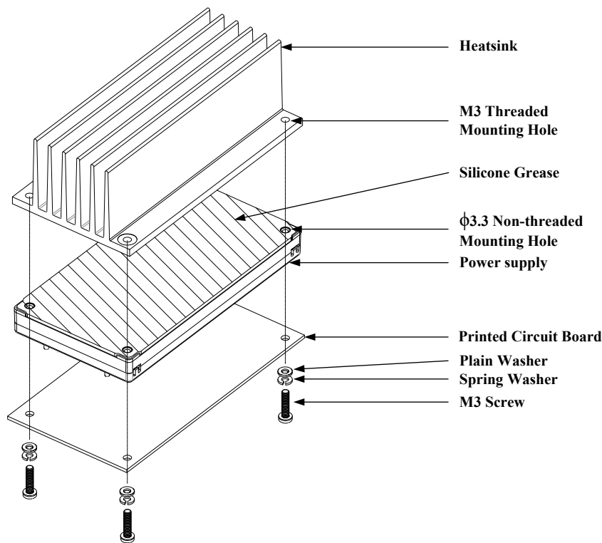
Fig.7-1 Mounting Method (b): /T option Mounting Method
