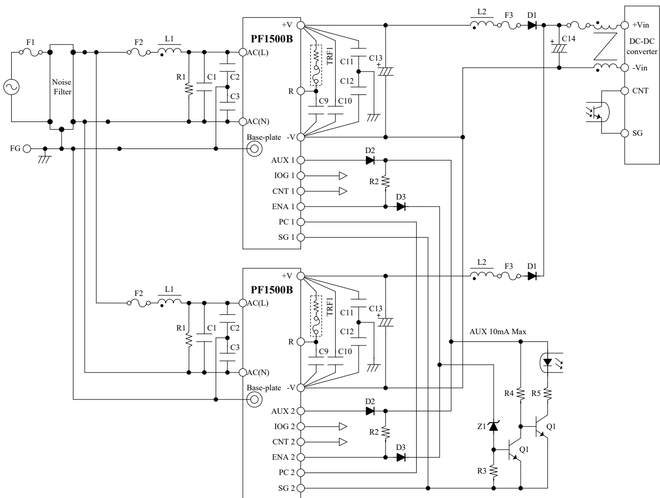
Fig.6-5 Basic Parallel Operation Connection
