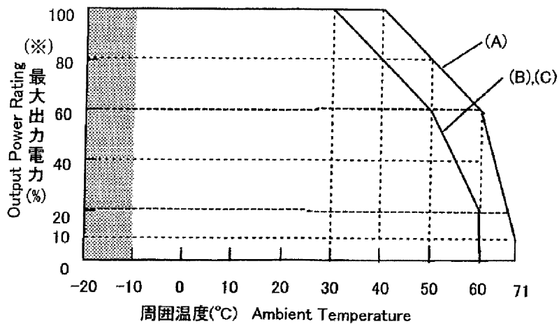
Fig-1 Power Derating Curve
