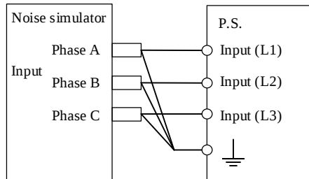
Common mode noise test
