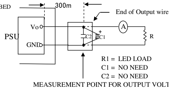
FIGURE A MEASUREMENT SETUP
