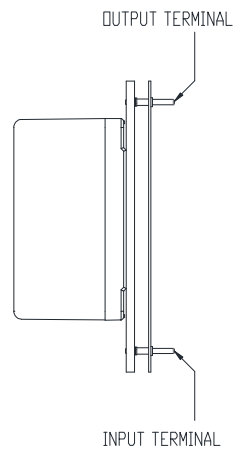
MOUNTING (E)
