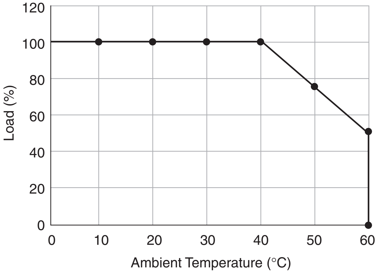
SCS120PW Series Derating Curve
