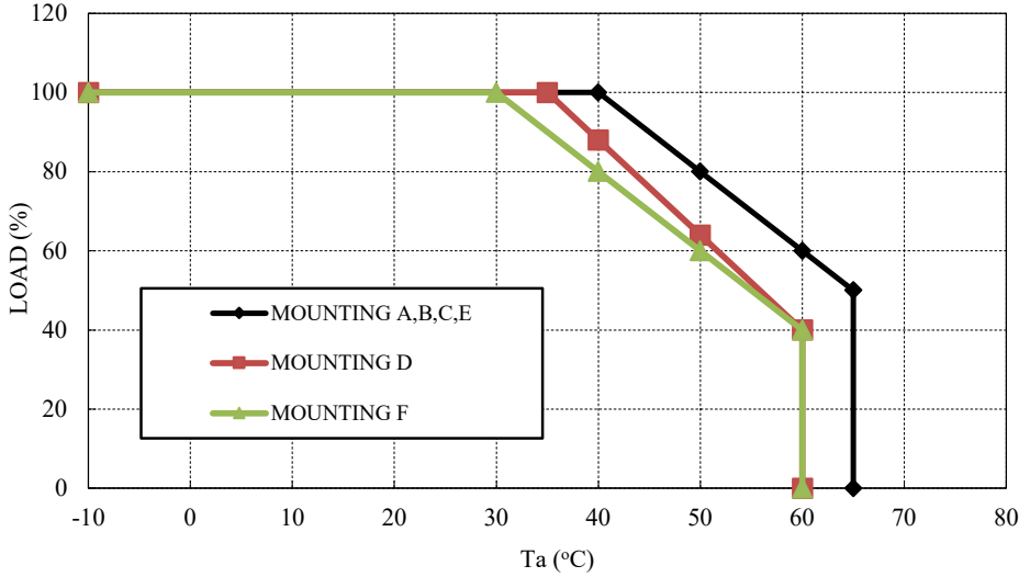
LOAD vs. AMBIENT TEMPERATURE (CONVECTION COOLING)
