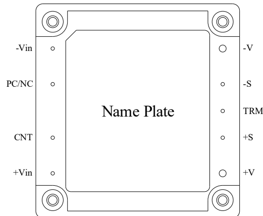
(b) CN200A
