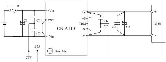
(a) CN30,50,100A
