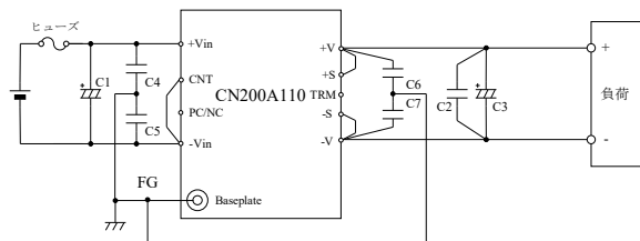
(b) CN200A
