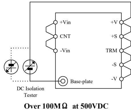
Fig.21-1 Isolation Resistance Test
