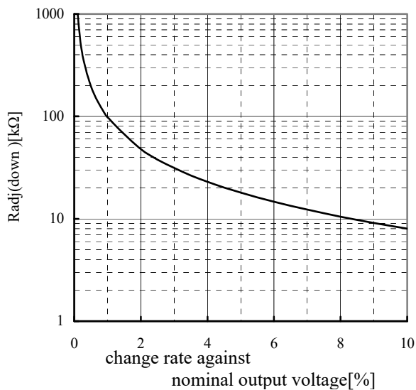
Fig.2-2 Δ(%) vs. Radj(down)
