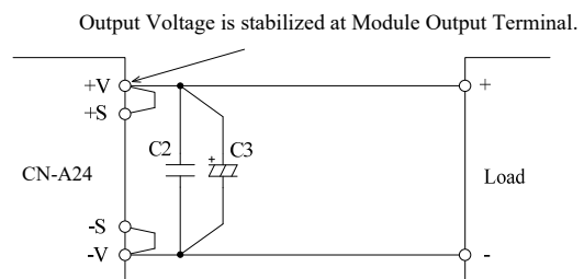
Fig.10-2 Remote Sensing is not used (Local Sensing)
