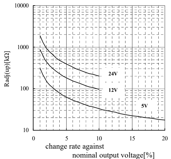
Fig.2-4 Δ(%) vs. Radj(up)
