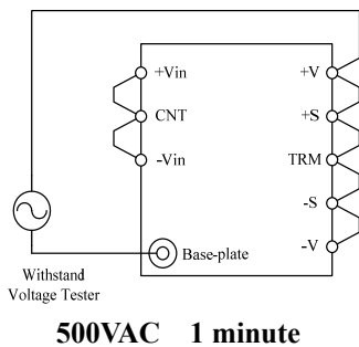
Fig.20-3 Withstand Voltage Test for Output – Base-plate
