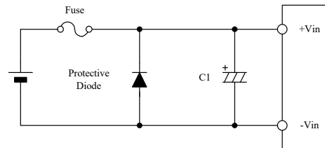
Fig.1-3 Protection for Reversed Connection of Input
