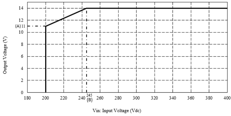
Fig.6-2 Limit of Input Voltage
