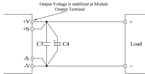
Fig.6-8 Remote Sensing Not in Use
