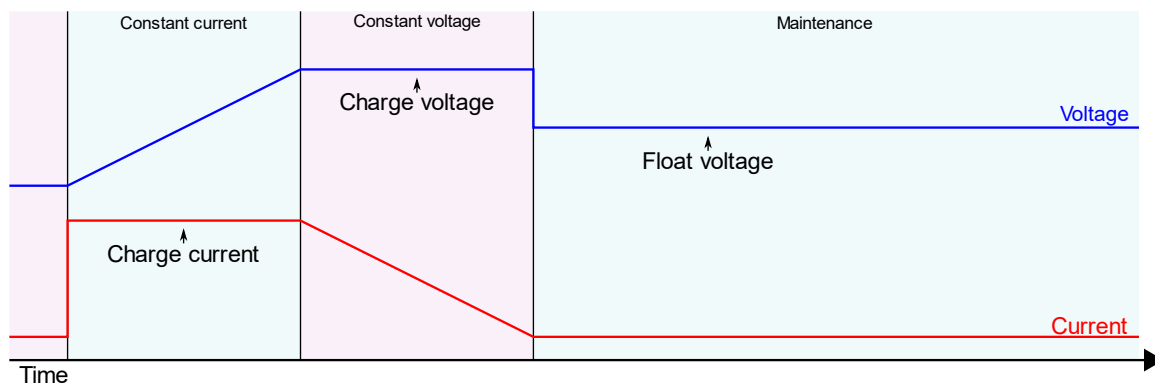
Figure 16 : Lead acid and Lithium charging algorithm
