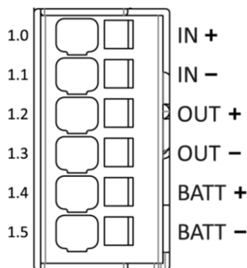
Figure 10 : Terminal block 1.x
