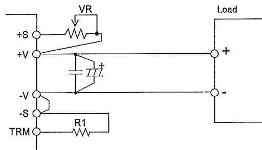
Fig.2-6 Example connection of external resistor
