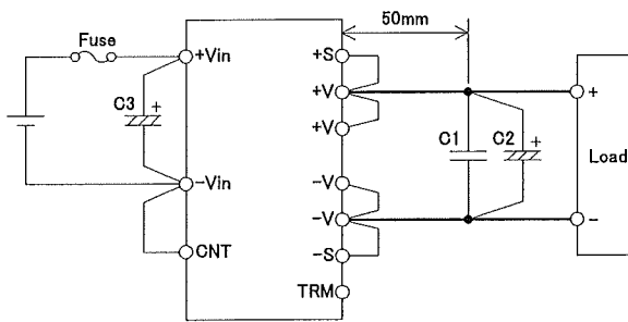
Fig.1-2 Basic Connection
