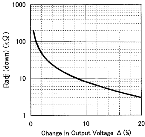
Fig.2-3 \Delta(\%) vs. R_{adj}(\text{down}) (1)
