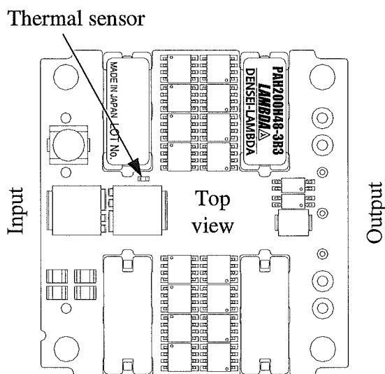
Fig.1-5 Thermal Sensor Position
