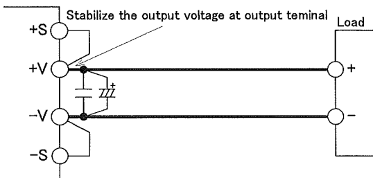
Fig.9-2 Remote Sensing Not in Use (Local Sensing)
