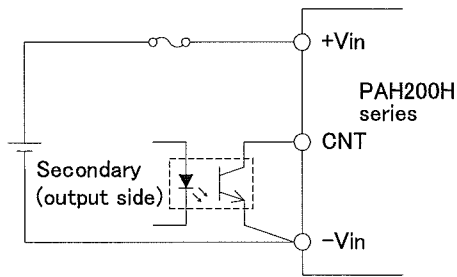
Fig.10-1 CNT Connection
