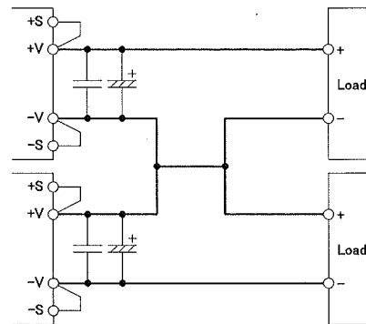
Fig.12-2 \pm Output Series Operation
