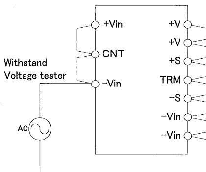
Fig.19-1 Withstand Voltage Test for Input-Output
