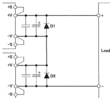
Fig.12-1 Series Operation for High Output Voltage
