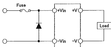
Fig.1-5 Protection for Reversed Input Connection
