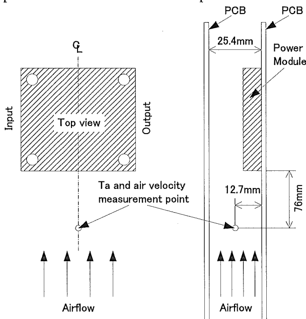
Fig.1-1 Output derating set-up condition
