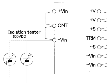
Fig.20-1 Isolated test
