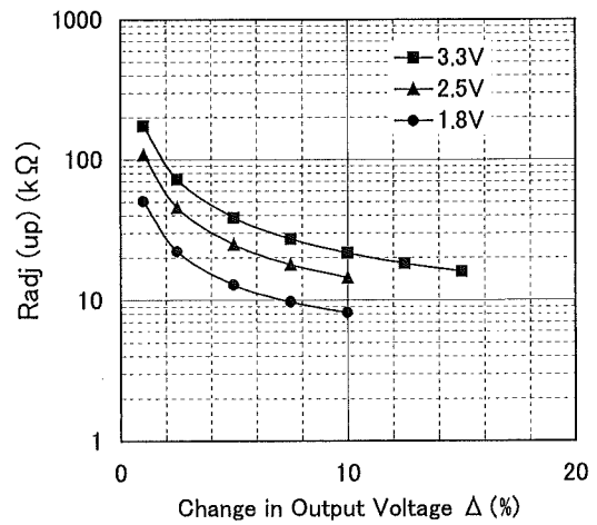
Fig.2-5 \Delta\% vs. R_{adj}(\text{up}) (2)
