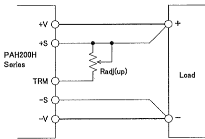
Fig.2-4 Connection for output voltage trim up(2)
