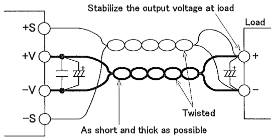
Fig.9-1 Remote Sensing in Use
