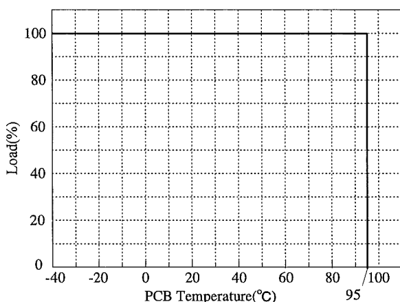
Fig.1-6 Output Derating by PCB Temperature
