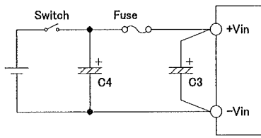
Fig.1-3 Input filter (C4) with Switch
