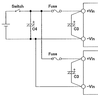
Fig.1-4 Input Filter with Switch when Plural Power
