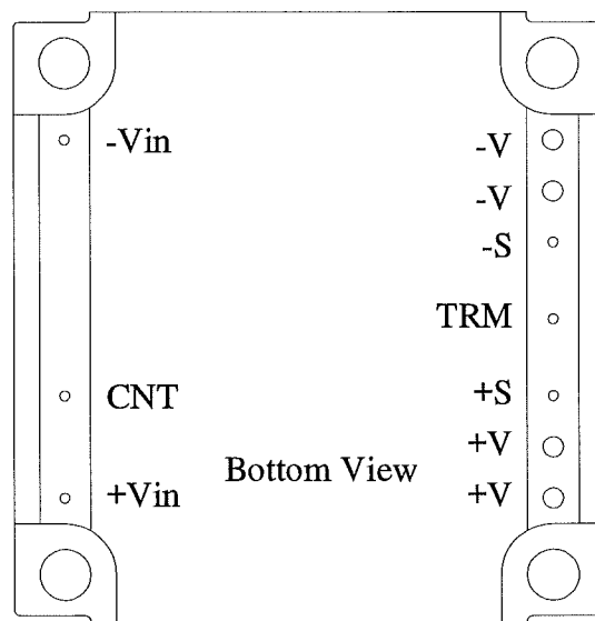
Input and Output Terminal Configurations (Bottom View)
