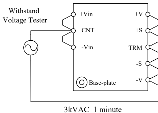
Fig.7-27 Withstand Voltage Test for Input – Output
