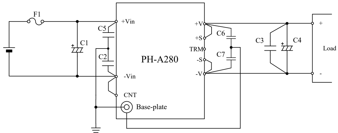
Fig.6-1 Basic connection
