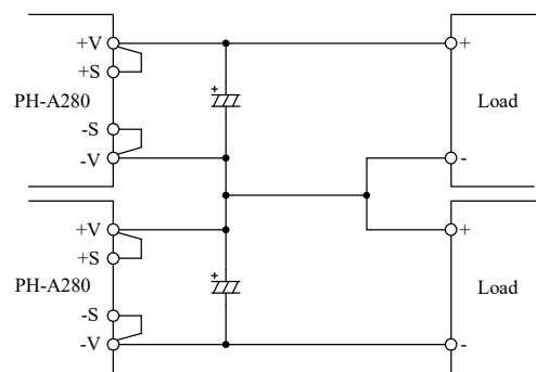
Fig.7-23 ±Output Series Operation
