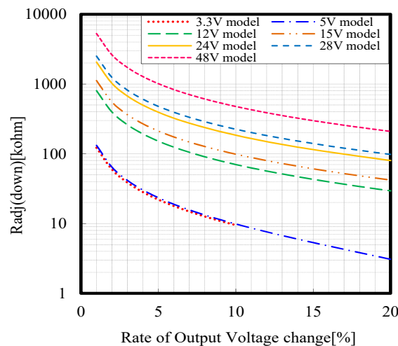
Fig.7-4 Radj(down) vs. Δ(%)
