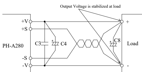
Fig.7-16 Remote Sensing is used
