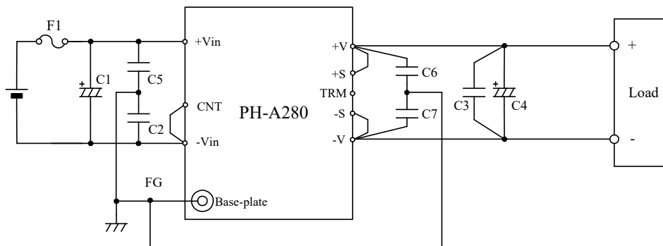
Fig.7-30 Example of connecting external application
