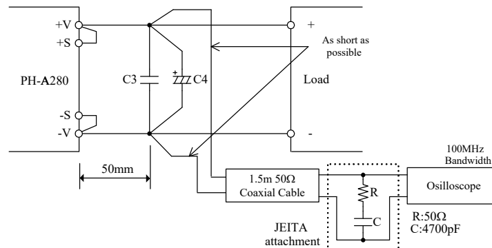
Fig.7-15 Measurement of Maximum Output Ripple and Noise
