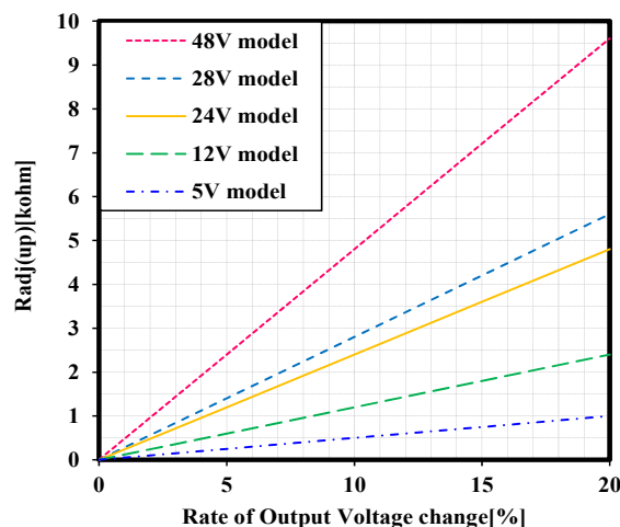
Fig.7-10 R adj(up) vs. Δ(%)
