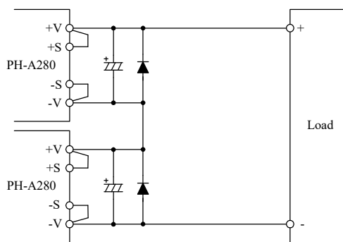
Fig.7-22 Series Operation for High Output Voltage
