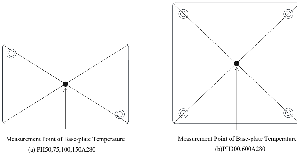
Fig.7-24 Measurement Point of Base-plate Temperature
