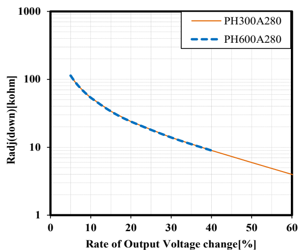
Fig.7-6 R adj(down) vs. Δ(%)
