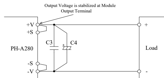
Fig.7-17 Remote Sensing is not used (Local Sensing)
