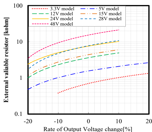
Fig.7-12 External Variable Resistor(VR) vs. Δ(%)
