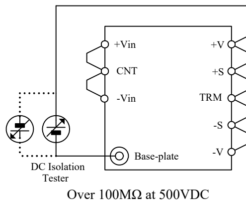
Fig.7-31 Isolation Resistance Test
