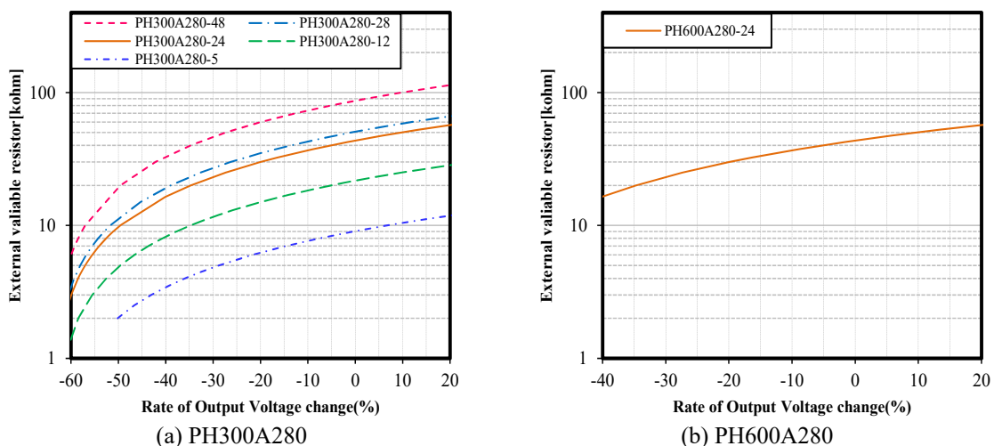
Fig.7-14 External Variable Resistor(VR) vs. Δ(%)
