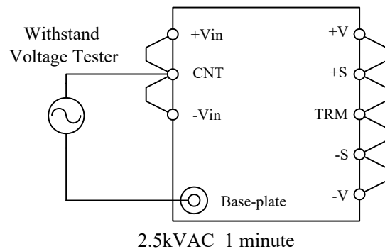
Fig.7-28 Withstand Voltage Test for Input – Base-plate
