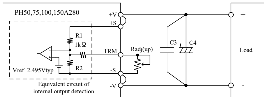
Fig.7-7 Connection for Output Voltage Trim Up
