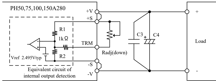
Fig.7-3 Connection for Output Voltage Trim Down
