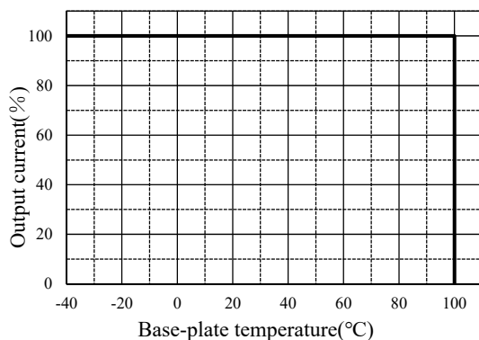
Fig.7-25 Derating Curve PH50,75,100,150,300A280
