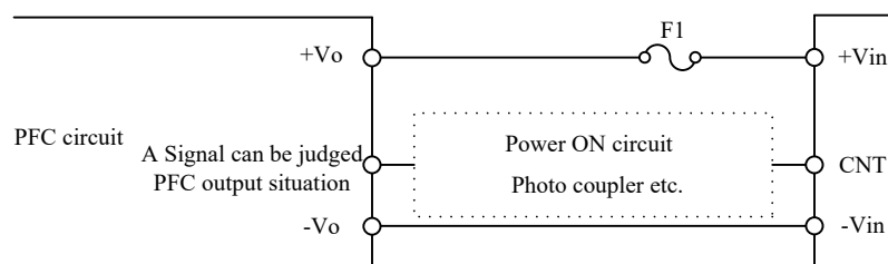
Fig.7-20 CNT Connection (3)
