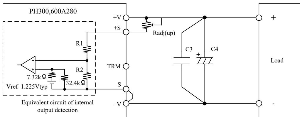
Fig.7-9 Connection for Output Voltage Trim Up
