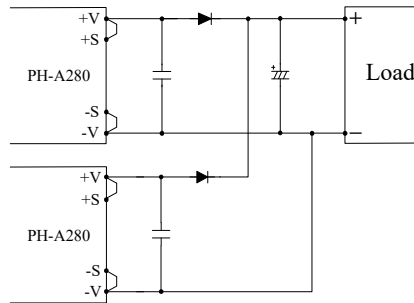
Fig.7-21 Redundant Operation Connection
