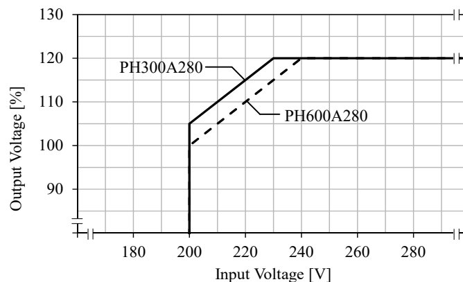
Fig.7-2 Limit of Input voltage
