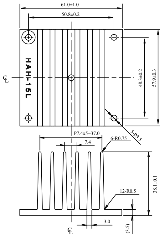
(2) HAH-15L (PH300,600A280)
