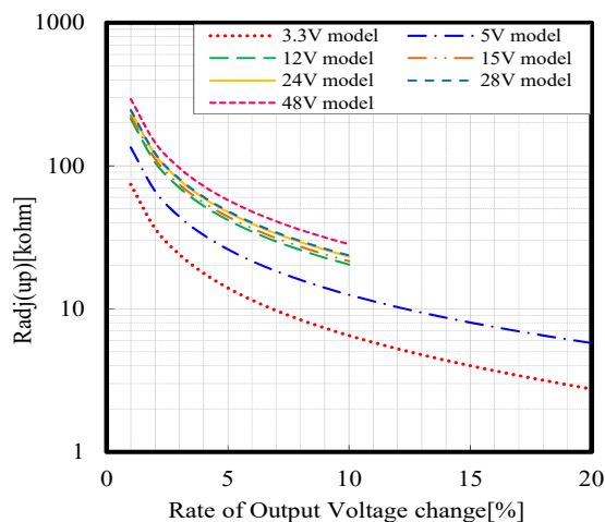
Fig.7-8 R adj(up) vs. Δ(%)
