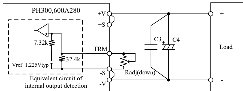
Fig.7-5 Connection for Output Voltage Trim Down
