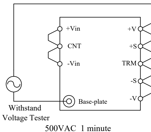
Fig.7-29 Withstand Voltage Test for Output – Base-plate
