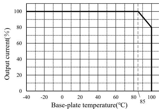
Fig.7-26 Derating Curve PH600A280
