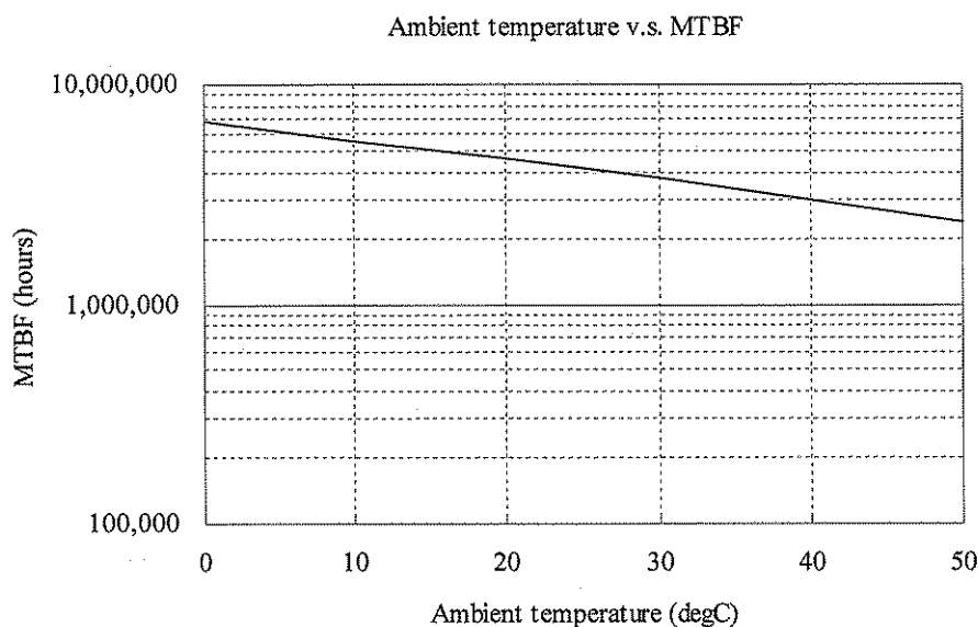
— PSD1R5-48-1212 Load 100%
