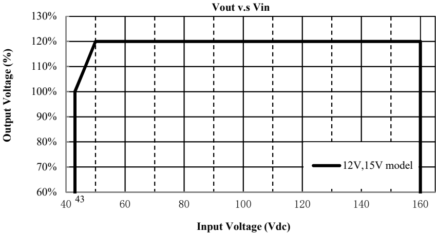
Derating Curve 2 Output Voltage Trim up Range Limited v.s Input Voltage
