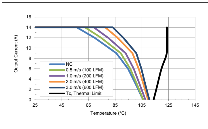
V_o = 18V , V_{in} = 24V preliminary maximum output current vs. ambient temperature at nominal input voltage for natural convection (60lfm) with airflow from pin 8 to pin 4.
