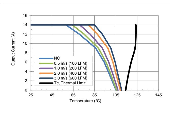
V_o = 12V , V_{in} = 24V preliminary maximum output current vs. ambient temperature at nominal input voltage for natural convection (60lfm) with airflow from pin 8 to pin 4.
