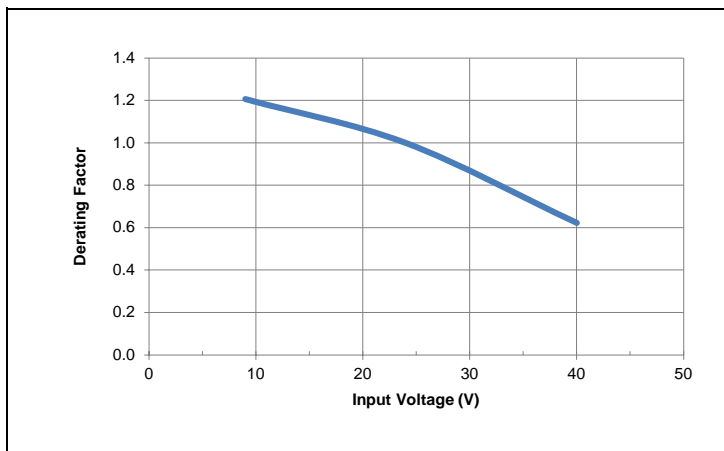
Typical ambient temperature derating versus line voltage with airflow 1m/s (200 lfm).
