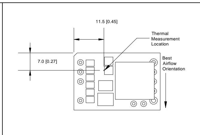
i6A24014A033V thermal measurement location – top view.
