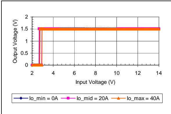
Vo=1.5V Typical Output Voltage vs. Input Voltage Characteristics
