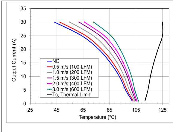
V_o=5.0V , V_{in}=12V maximum output current vs. ambient temperature at nominal input voltage for natural convection (60lfm) with airflow from pin7 to pin 3.
