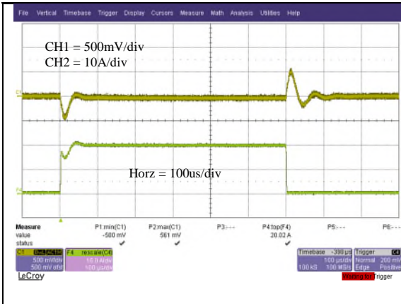
Vo=1.8V Typical output voltage transient response to load step from 25% to 75% of full load with output current slew rate of 10A/uS. (Cext = 4x47uF ceramic capacitor)
