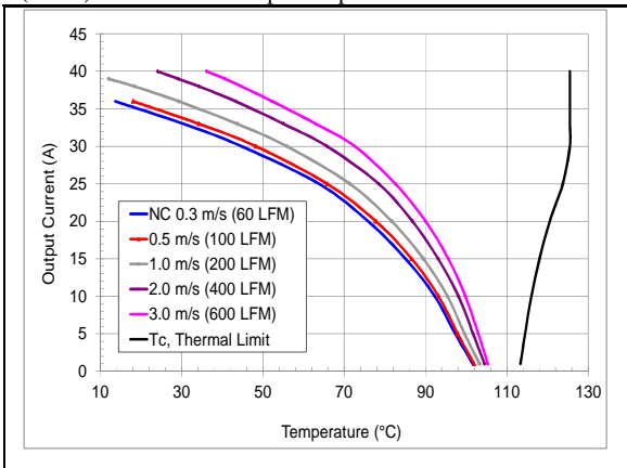
V_o=1.8V , V_{in}=12V maximum output current vs. ambient temperature at nominal input voltage for natural convection (60lfm) with airflow from pin 7 to pin 3.
