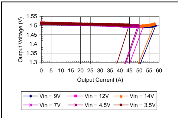
Vo=1.5V Typical Current Limit Characteristics
