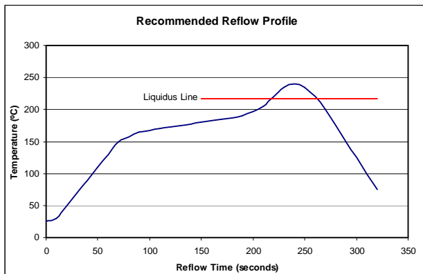
iAH Power Module suggested reflow-soldering profile
