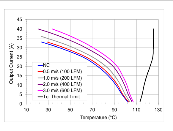
V_o=3.3V , V_{in}=12V maximum output current vs. ambient temperature at nominal input voltage for natural convection (60lfm) with airflow from pin 7 to pin 3.
