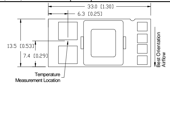
iAH12040A007V thermal measurement location – top view
