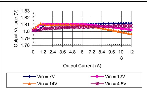
Vo=1.8V Typical load regulation
