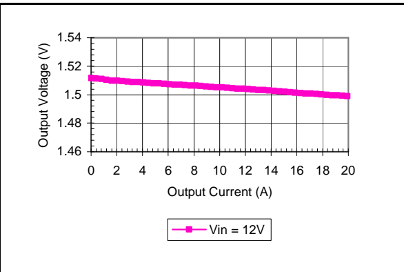
Vo=1.5V Typical load regulation
