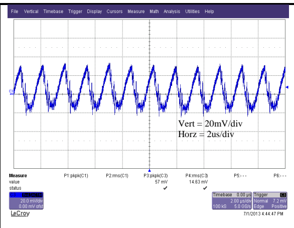
Vo=1.8V Typical Input Ripple at nominal Input Voltage and full load at Ta=25 degrees. Input capacitors 6 x 22uF ceramic
