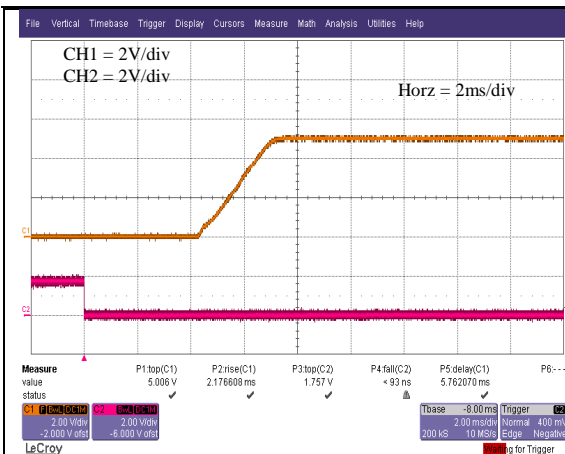
Vo=5V Typical startup characteristic from on/off at full load. Ch1 - output voltage, Ch2 - on/off signal
