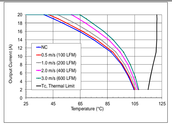
V_o=3.3V , V_{in}=12V maximum output current vs. ambient temperature at nominal input voltage for natural convection (60lfm) with airflow from pin 2 to pin 3.
