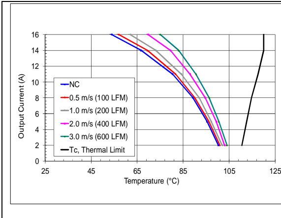
V_o=5.0V , V_{in}=12V maximum output current vs. ambient temperature at nominal input voltage for natural convection (60lfm) with airflow from pin 2 to pin 3.
