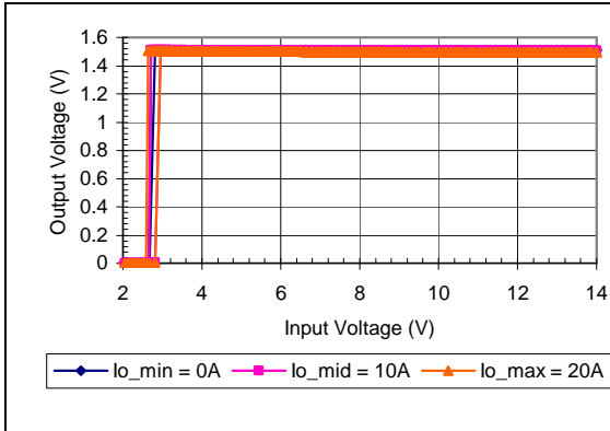
Vo=1.5V Typical Output Voltage vs. Input Voltage Characteristics
