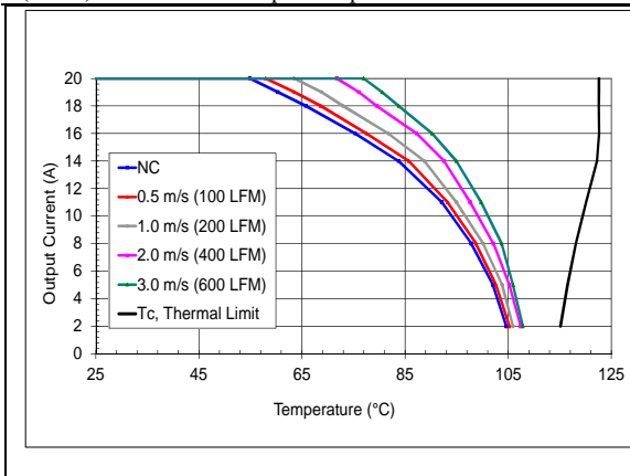
V_o=1.8V , V_{in}=12V maximum output current vs. ambient temperature at nominal input voltage for natural convection (60lfm) with airflow from pin 2 to pin 3.
