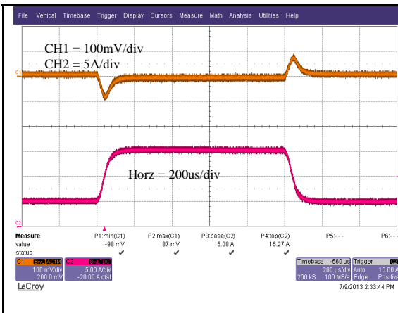
Vo=1.8V Typical output voltage transient response to load step from 25% to 75% of full load with output current slew rate of 0.25A/uS. (Cext = 4x47uF ceramic capacitor)
