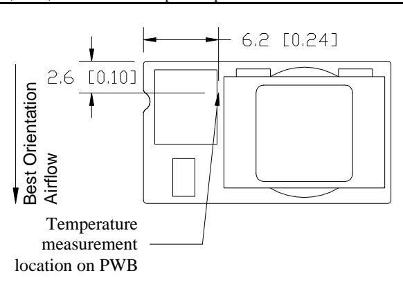
iBH12020A007V thermal measurement location – top view
