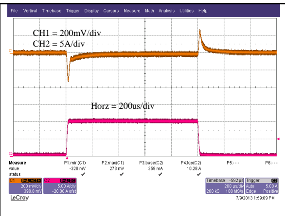
Vo=3.3V Typical output voltage transient response to load step from 0% to 50% of full load with output current slew rate of 1A/uS. (Cext = 4x47uF ceramic capacitor)
