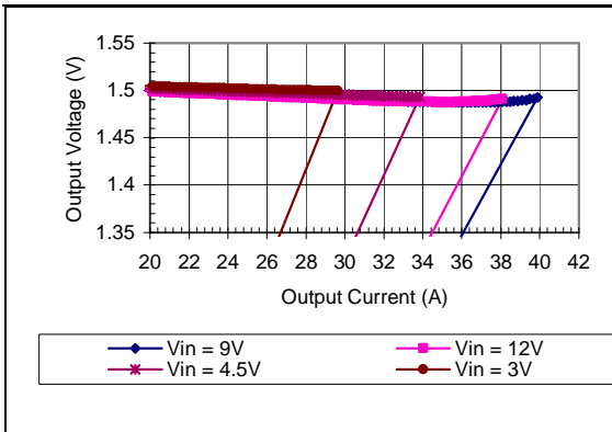
Vo=1.5V Typical Current Limit Characteristics
