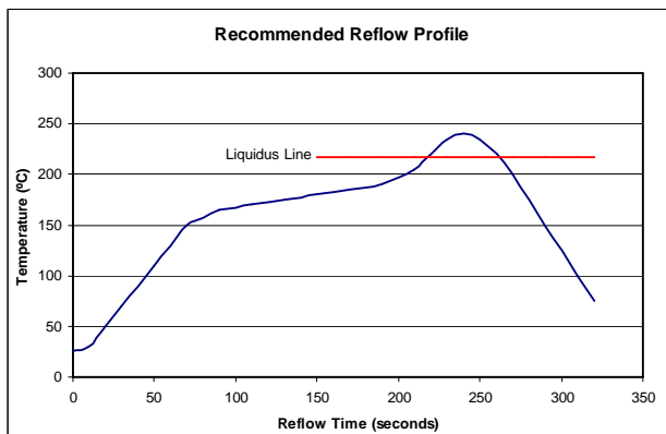
iBH Power Module suggested reflow-soldering profile
