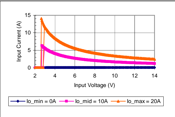
Vo=1.5V Typical Input Current vs. Input Voltage Characteristics
