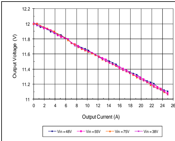
Typical Output Voltage vs. Load Current at Ta=25C (Droop Feature Enabled)
