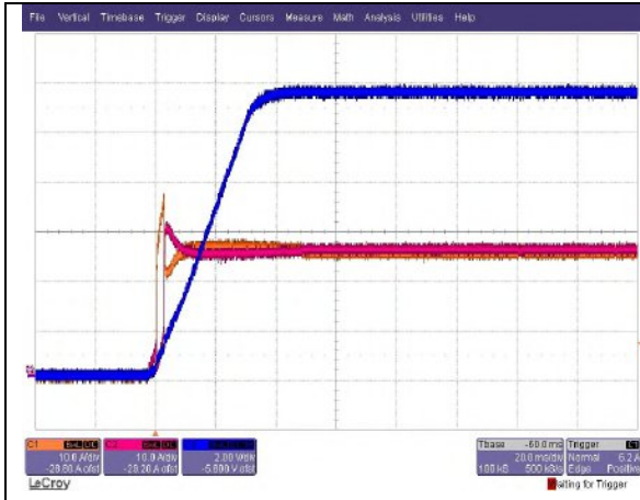
Start-up from on/off switch: 48Vin, Io=50A (200% Load) Ch. 1: Io1 Ch. 2: Io2 Ch. 3: Vo
