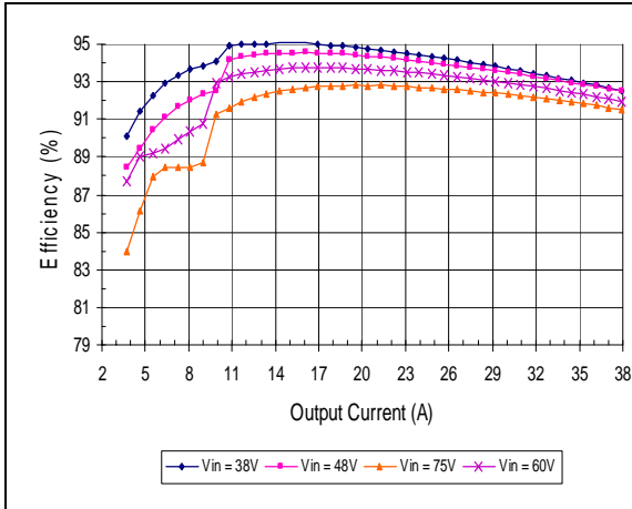
Efficiency vs. Vin at Ta=25°C (test in socket)
