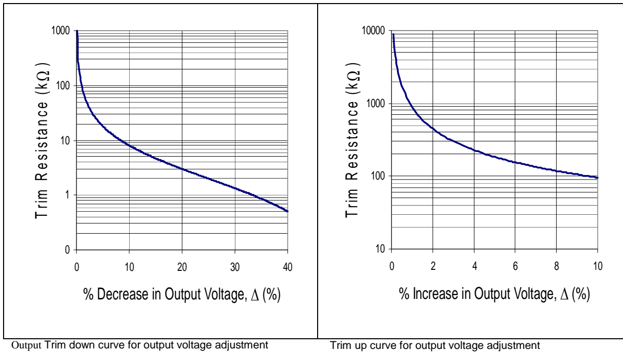
Output Trim down curve for output voltage adjustment
