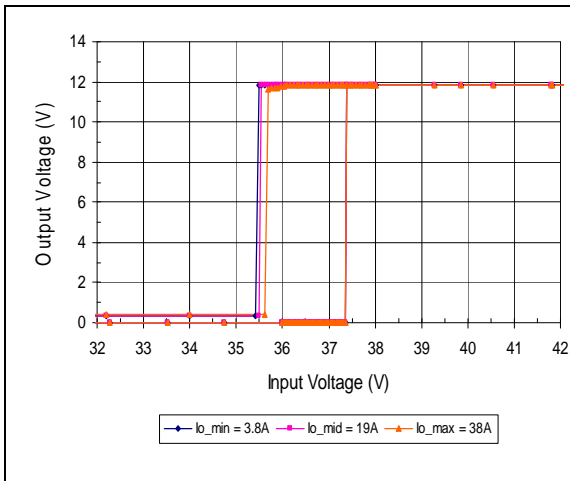
Typical Output Voltage vs. Low Voltage Input Turn-on and Turn-off at Ta=25°C
