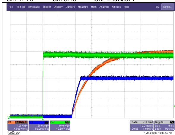
Start-up from Input Voltage Application at Full Load. Ch. 2: Vo Ch. 3: Io Ch. 4: Vin
