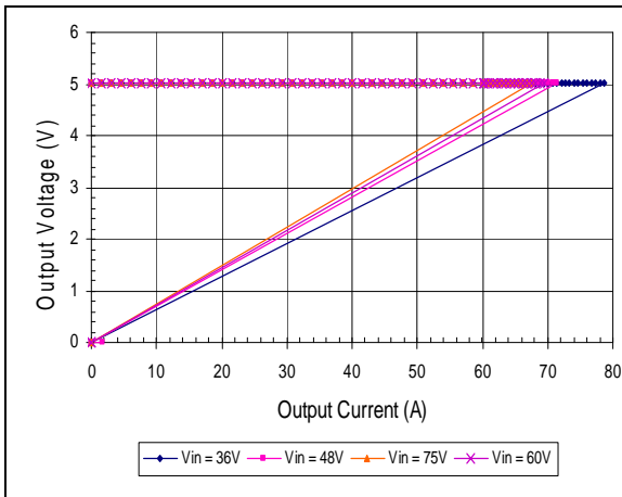
Output Current Limit Characteristics vs. Input Voltage
