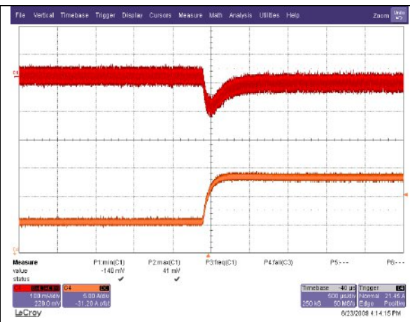
Load Transient Response. Load Step from 50% to 75% of Full Load with di/dt= 0.1A/uS. Ch. 1: Vo Ch. 4: Io
