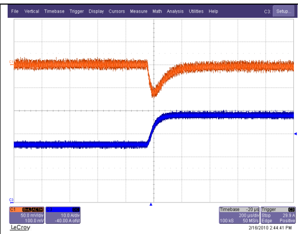
Load Transient Response. Load Step from 50% to 75% of Full Load with di/dt= 0.1A/μs. Ch. 1: Vo Ch. 3: Io
