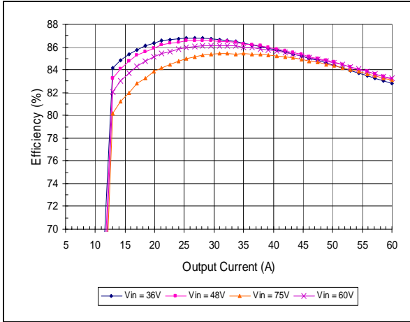
Efficiency vs. Vin (test in socket without a base-plate)
