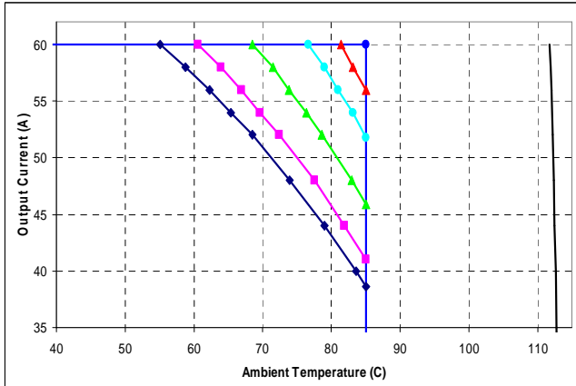
Maximum output current vs. ambient temperature at nominal input voltage with base plate for airflow rates natural convection (0.3m/s) to 3.0m/s with airflow from pin 3 to pin 1.
