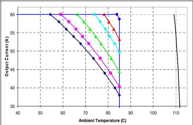
Maximum output current vs. ambient temperature at nominal input voltage with base plate for airflow rates natural convection (0.3m/s) to 3.0m/s with airflow from pin 1 to pin 3.
