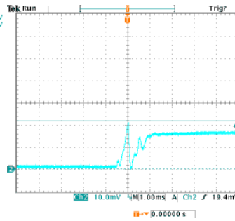
High Line, Full Load Inrush current=(21.6/10) x200mA=432mA
