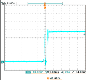
Low Line, Full Load Duration: 240uS
