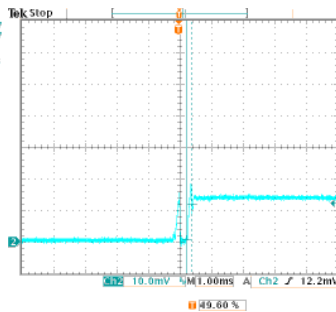
Normal Line, Full Load Duration: 180uS
