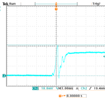
Normal Line, Full Load Inrush current=(31.0/10) x200mA=620mA
