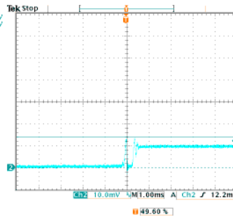
High Line, Full Load Inrush current=(13.8/10) x500mA=690mA
