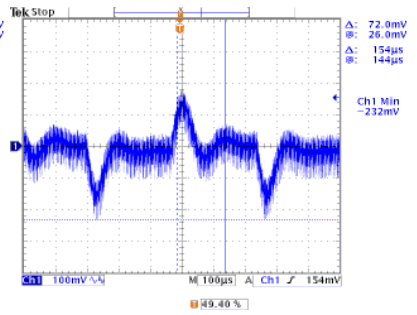
High Line, Full Load Transient Peak 232mV Transient Response 154µs
