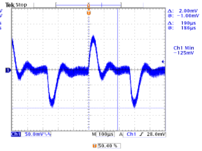
High Line, Full Load Transient Peak 125mV Transient Response 190µs
