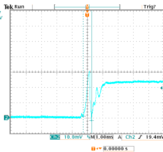
Normal Line, Full Load Duration: 540uS
