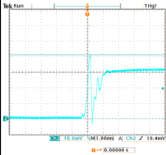
Low Line, Full Load Inrush current=(41.0/10) X200mA=820mA
