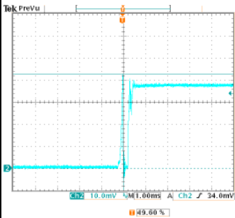
Low Line, Full Load Inrush current=(42.8/10) X500mA=2140mA
