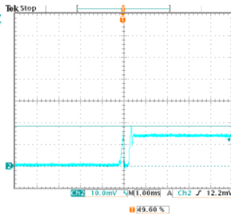
Normal Line, Full Load Inrush current=(18.4/10) x500mA=920mA
