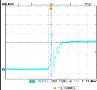
Low Line, Full Load Duration: 600uS
