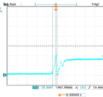
High Line, Full Load Duration: 520uS
