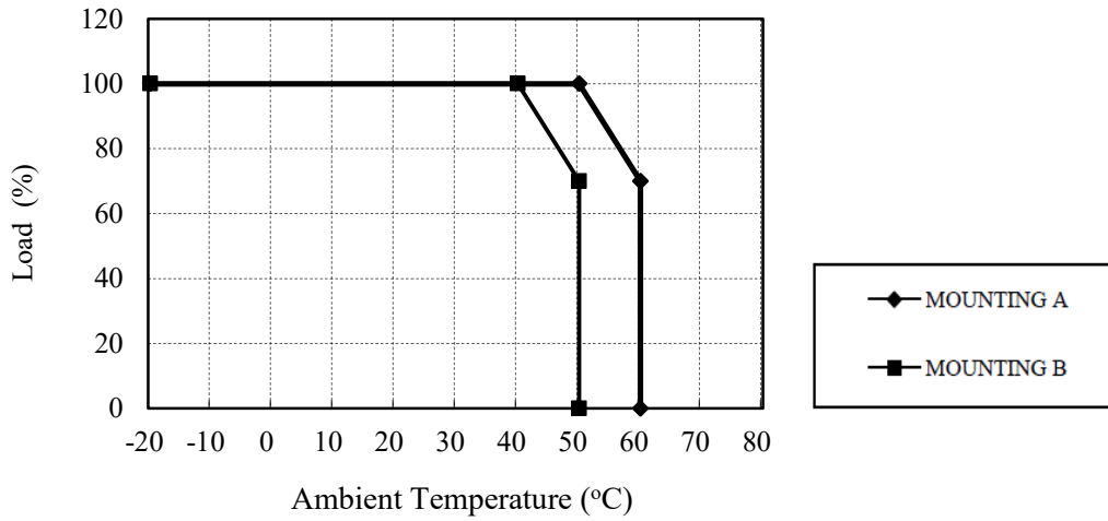
Derating Curve
