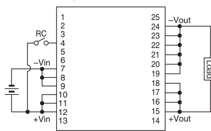
Connection diagram
