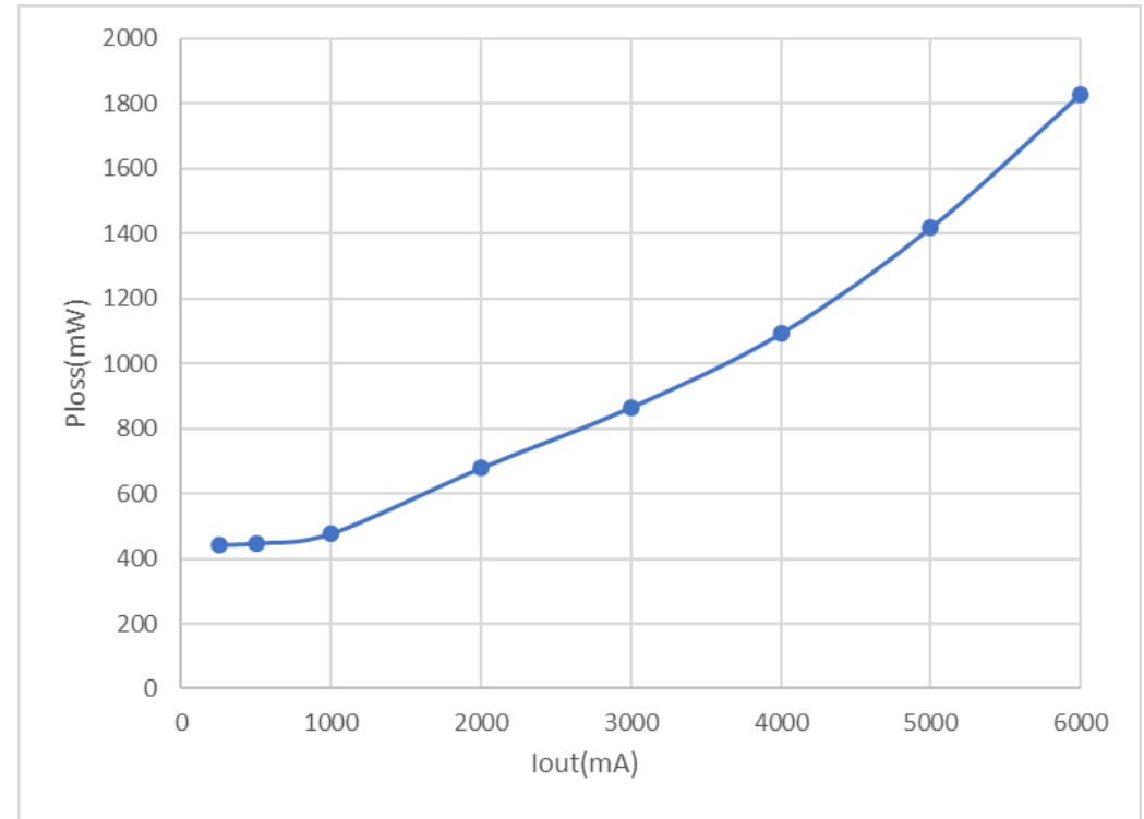
Power Loss
