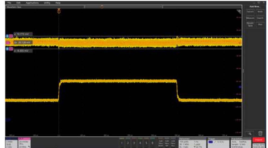
Load transient 3A-6A
