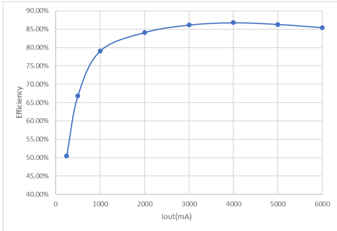
Efficiency
