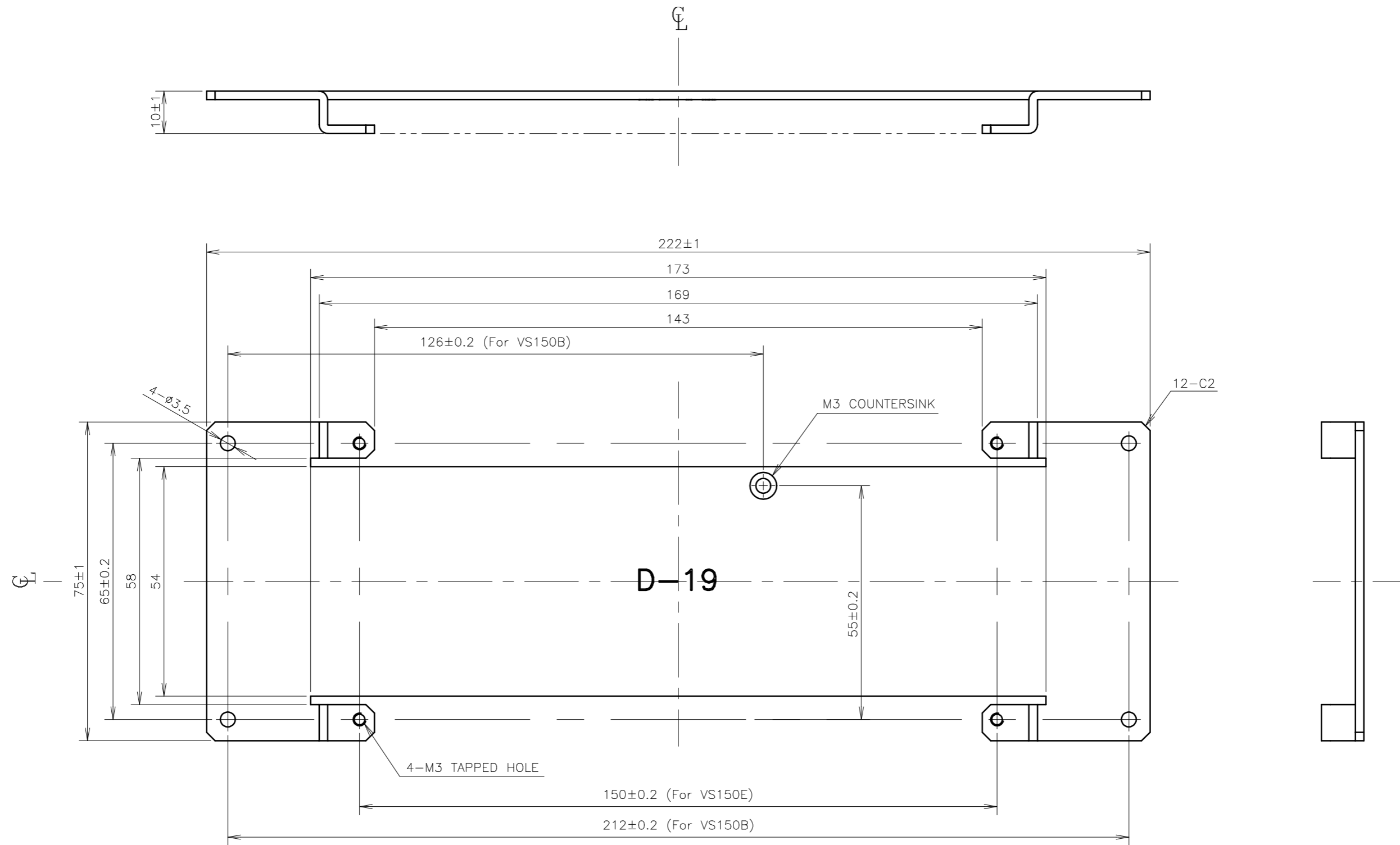
Mounting Plate for VS150B=>VS150E
