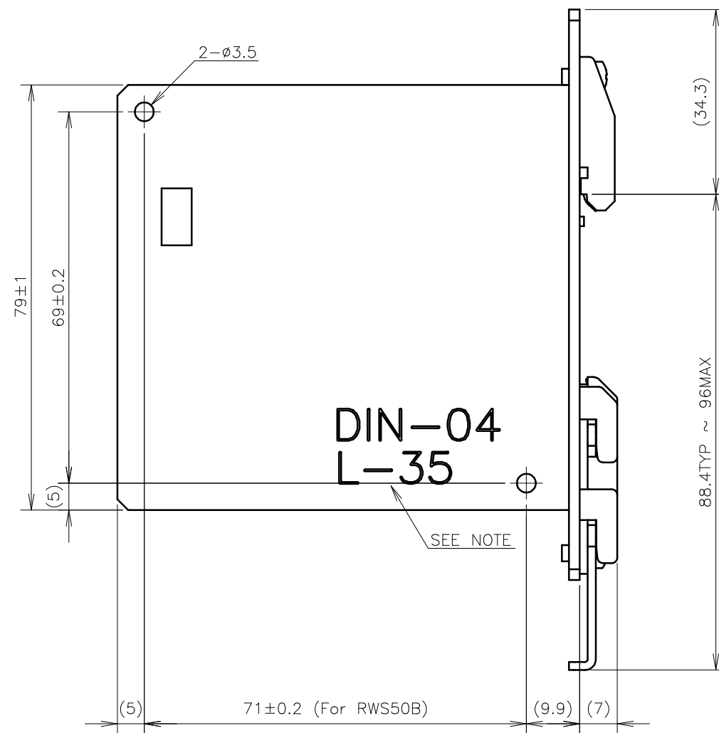
Mounting Plate for RWS50B
