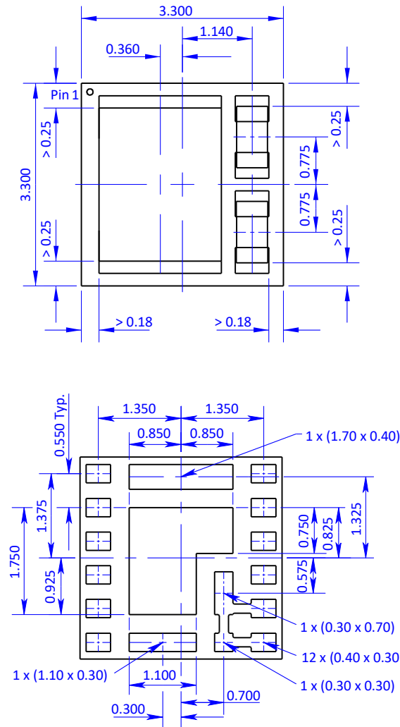
Figure 19 Dimensioned drawings
