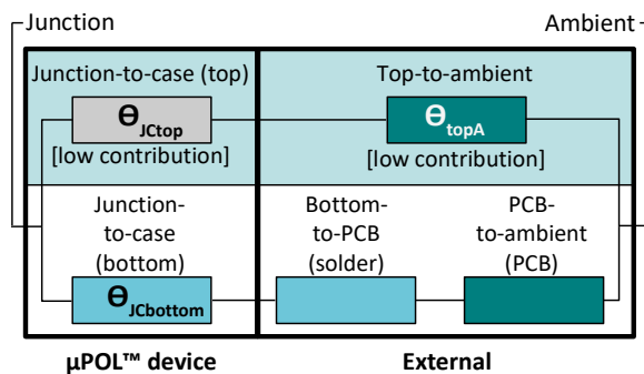
Figure 18 Thermal resistances of the FS1604A
