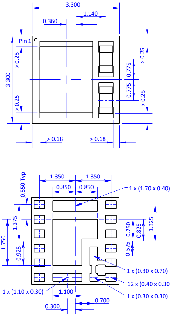
Figure 19 Dimensioned drawings
